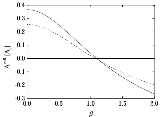
FIG. 1. Dynamic part of Hamaker constant as a function of \beta = n_1/n_{2\perp} . Solid line corresponds to uniaxial and the dashed line to isotropic Hamaker constant in units of A_0 = 3\hbar\omega_e n_{2\perp}/8\sqrt{2} . Here, n_{2\parallel}/n_{2\perp} = 1.2 and n_3/n_{2\perp} = 0.67 .
