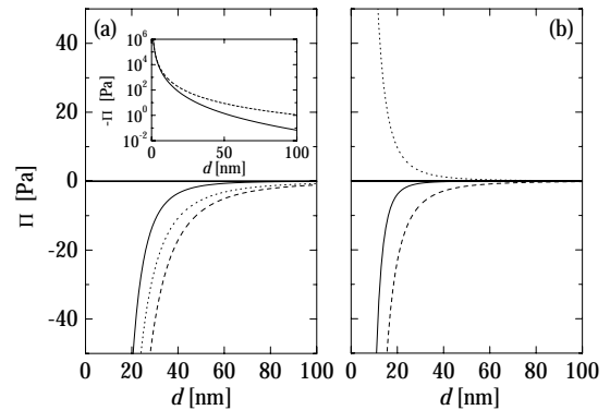
FIG. 2. Van der Waals force per unit area in the layer of nematic liquid crystal in a contact with a solid substrate — (a) silica ( \epsilon = 14 , n = 1.5 ), (b) mica ( \epsilon = 11 , n = 1.6 ) — and air. Solid curves correspond to full Lifshitz theory for uniaxial media, dashed curves are the van der Waals force per unit area calculated with uniaxial Hamaker constant, and dotted lines are calculated with Hamaker constant for isotropic media. Inset: logarithmic plot of uniaxial pressures.
